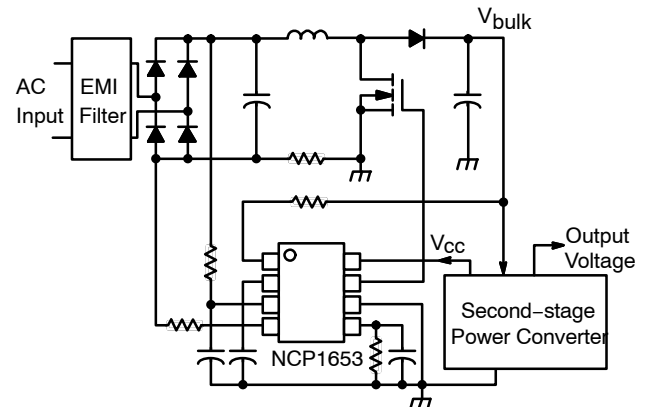
Figure 39. Recommended Biasing Scheme in Follower Boost Mode
