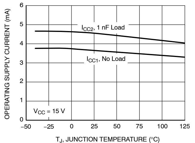
Figure 24. Operating Supply Current vs. Temperature
