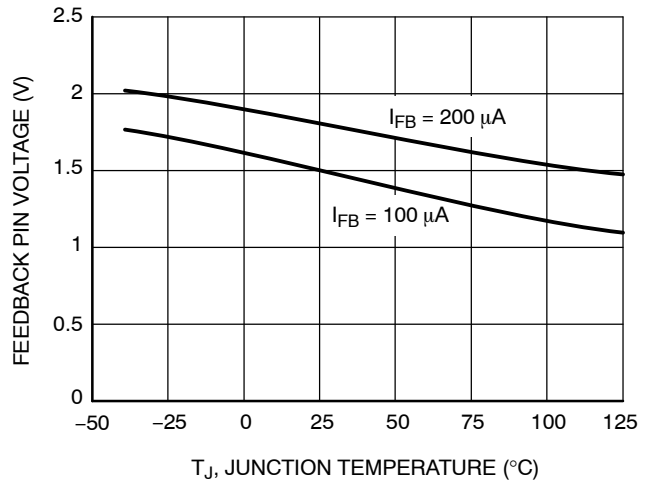
Figure 10. Feedback Pin Voltage vs. Temperature
