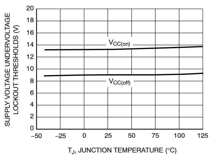
Figure 22. Supply Voltage Undervoltage Lockout Thresholds vs. Temperature
