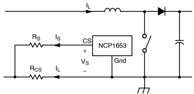
Figure 36. Current Sensing
