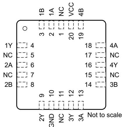
SN54HC08 FK Package 20-Pin LCCC Top View
