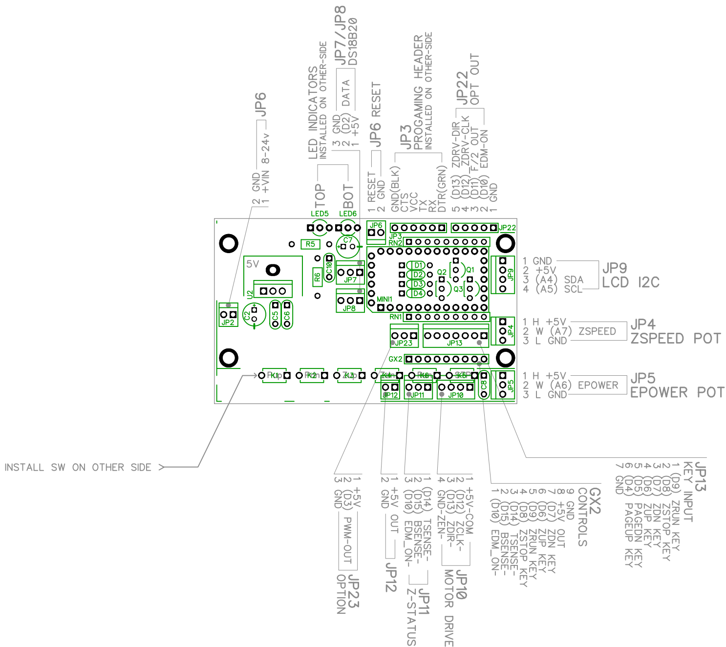
CES181005-1_v01 PCB ASSEMBLY ZDRV ONLY W/ ON-BOARD KEY FOR 1602 LCD DISPLAY
