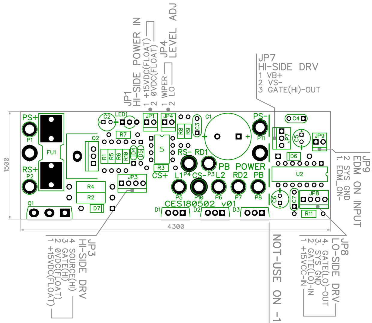
CES180502-6 v01 EDM PB POWER BOARD
