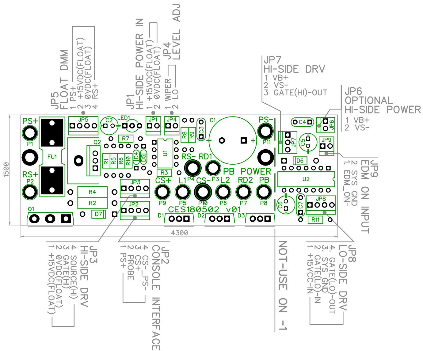
CES180502-2 v01 EDM PB POWER BOARD
