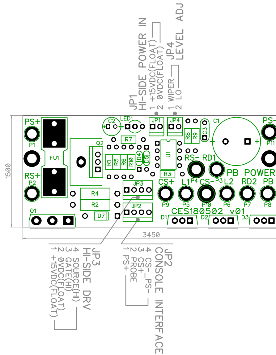
CES180502-1 v01 EDM PB POWER BOARD
