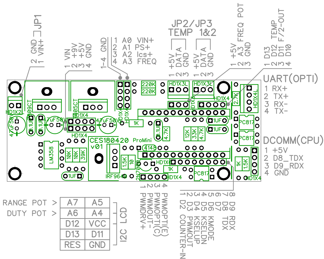
CES180420-N_v01 PCB ASSY
