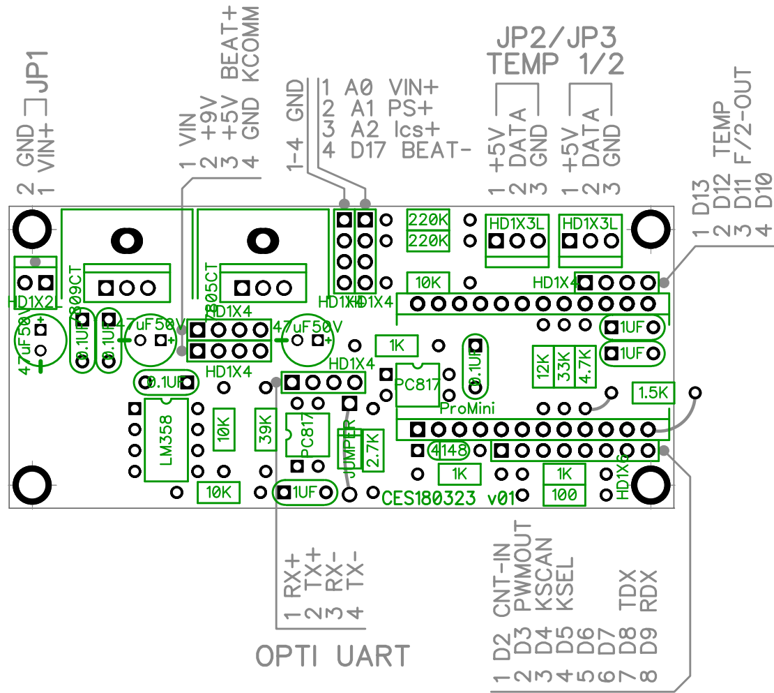
CES180323-N PCB ASSY
