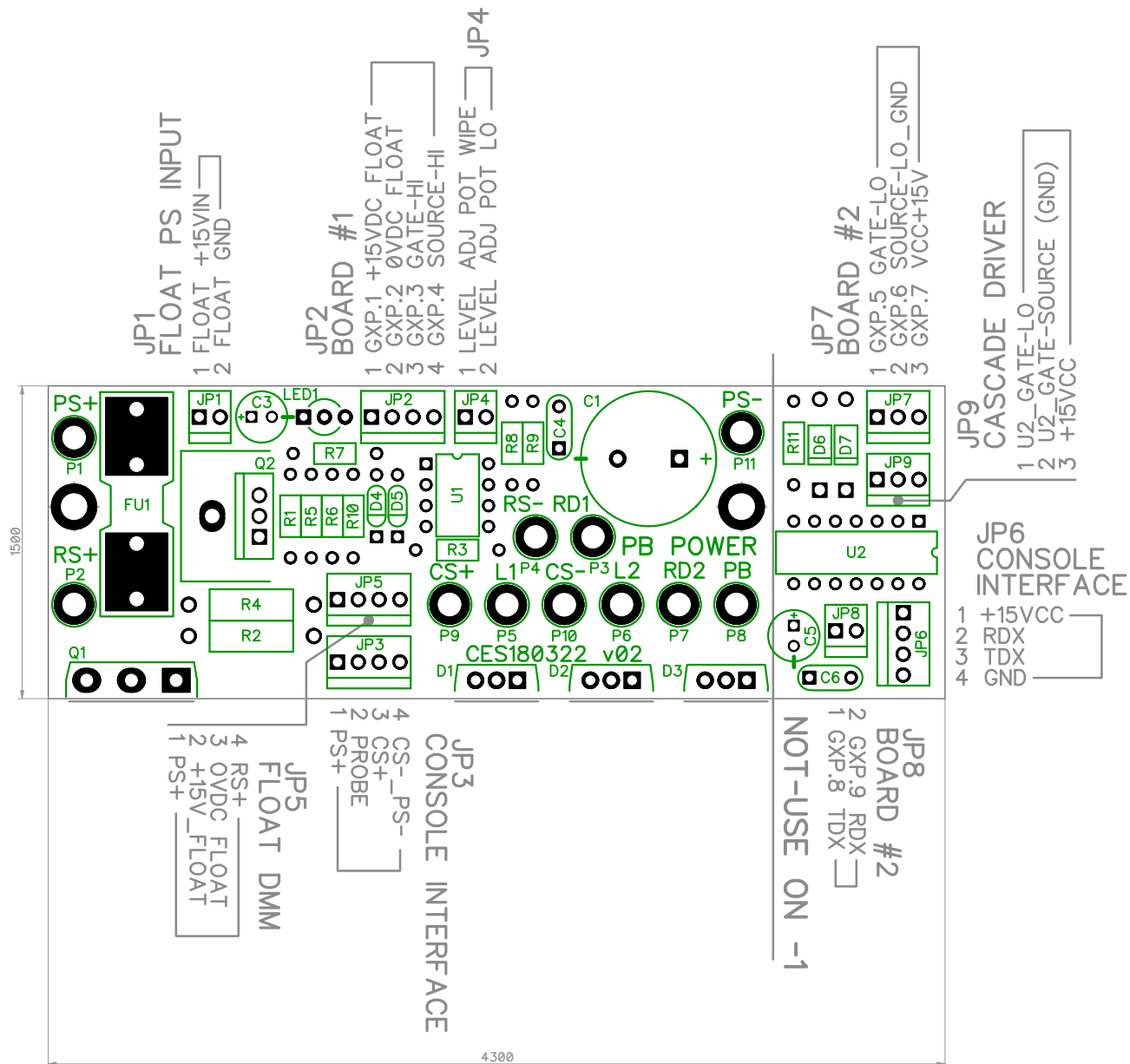
CES180322 EDM PB POWER BOARD
