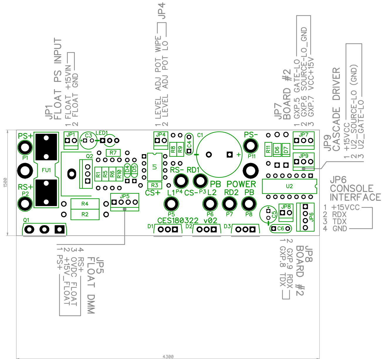
CES180322-4 EDM PB POWER BOARD 15A LO-SIDE POWER w/ Lo-Side Cascade Driver
