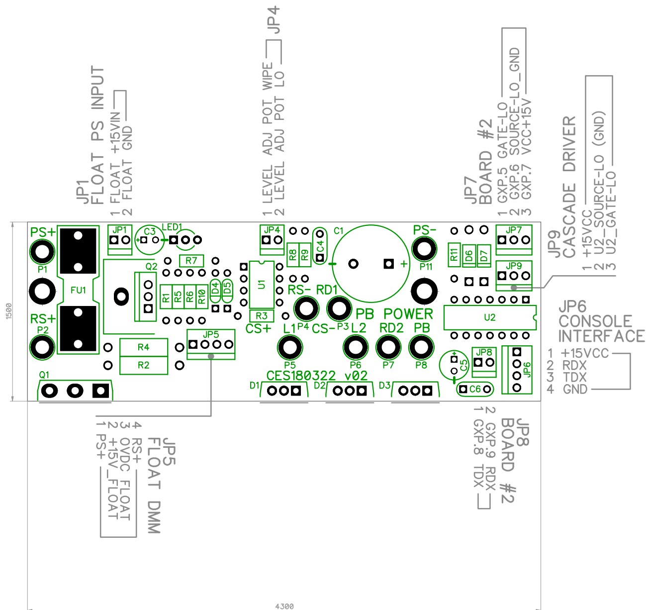
CES180322-2 EDM PB POWER BOARD 15A LO-SIDE POWER w/ Lo-Side Cascade Driver
