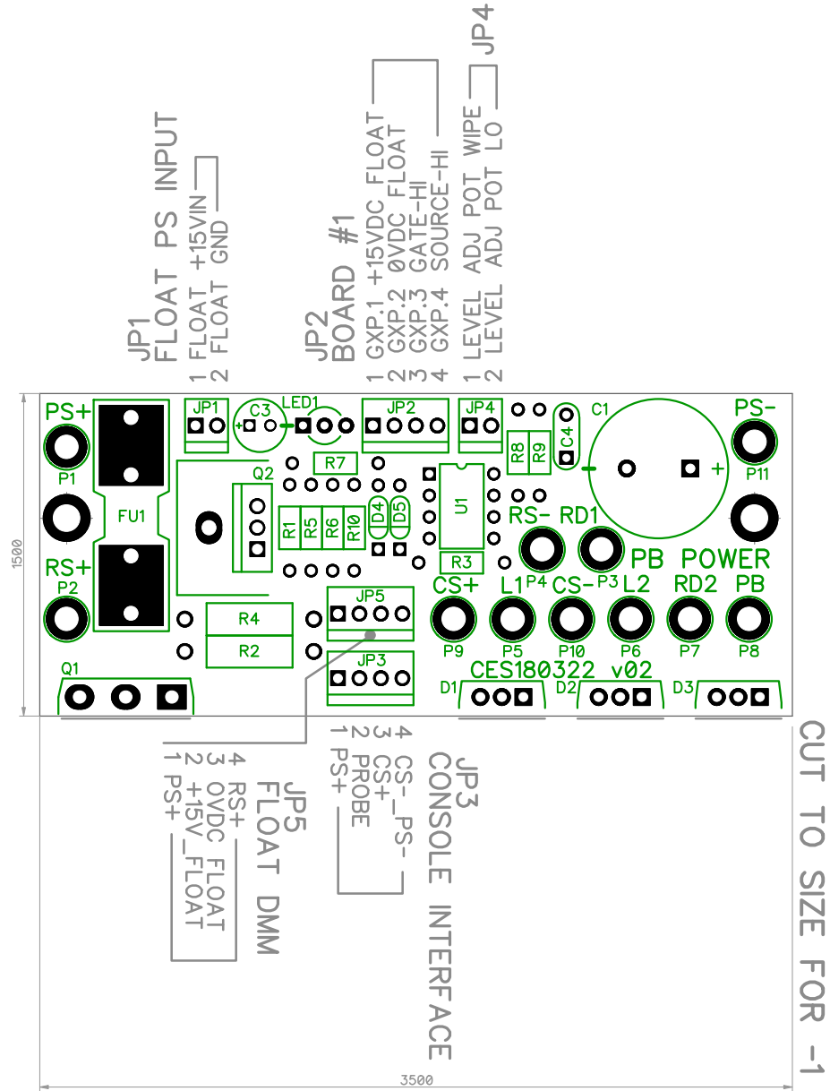
CES180322-1 EDM PB POWER BOARD 15A HI-SIDE ONLY
