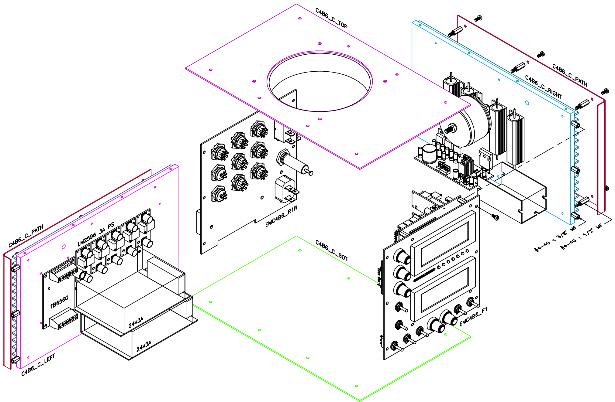
EMC4_BOX6_ASSY
